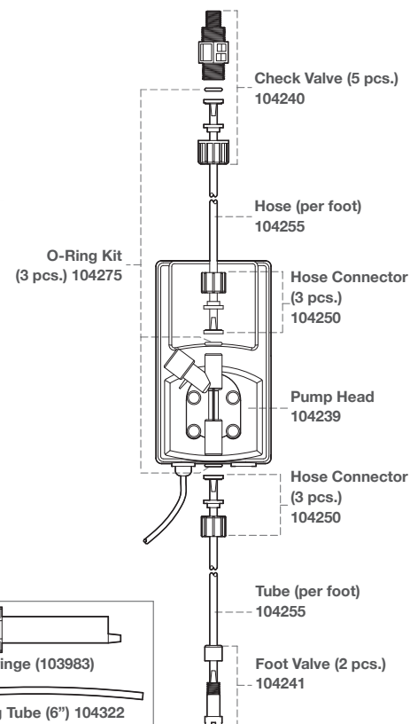
AromaSteam Metering Pump "E" Style
