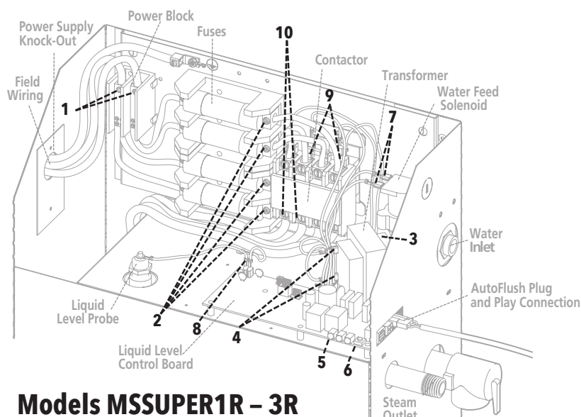
Models MS90R – MS400R (single phase wiring shown)
