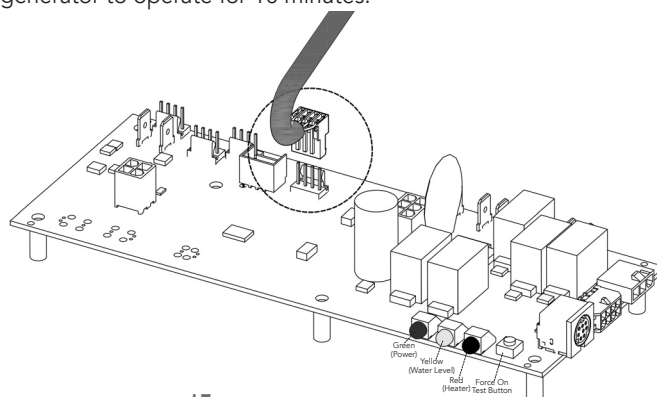
Circuit Board PN 104724 (shown without wiring)
