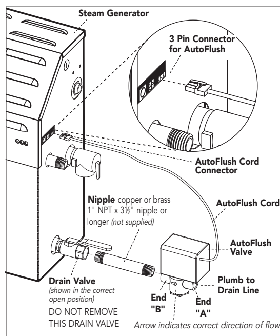
AutoFlush Shown Fully Assembled
