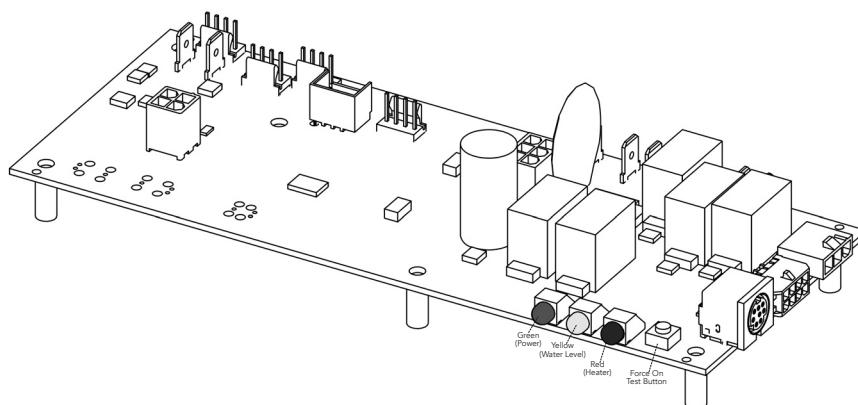
Liquid Level Control Board PN 104724 (shown without wiring)
