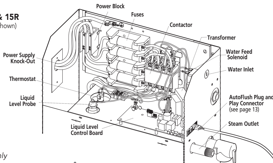
Models CT6R (single phase wiring shown)
